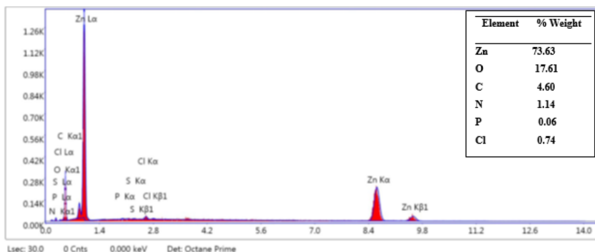
Fig. 5: EDX spectrum of the biosynthesized ZnO.
