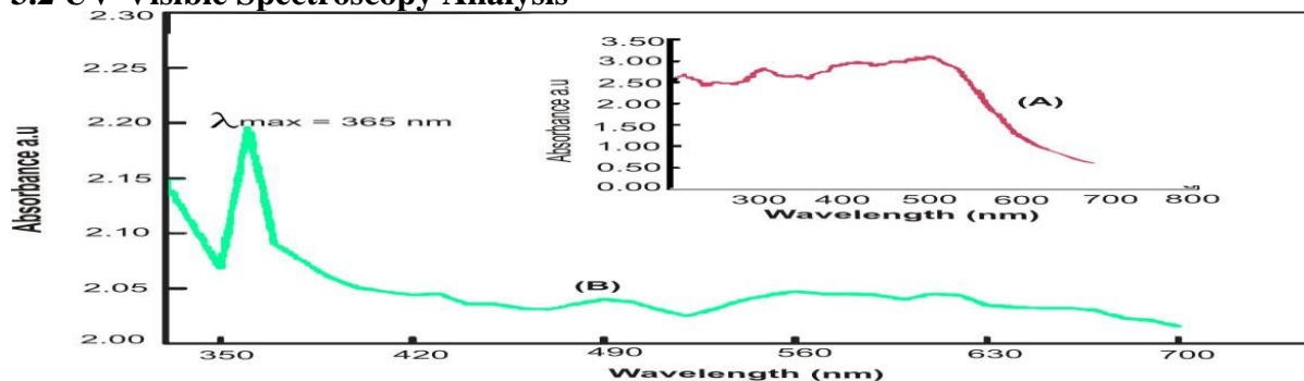
Fig. 2. UV-Vis spectra of (A) Colocasia esculenta leaves extract and (B) the biosynthesized ZnO NPs recorded as a function of reaction time.
