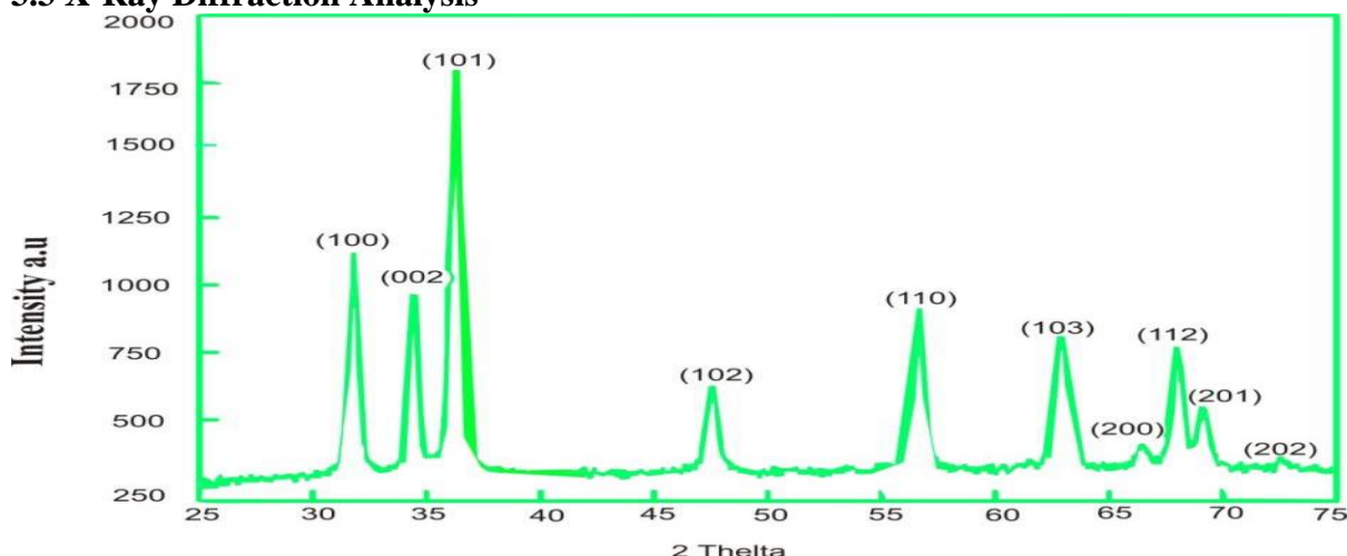
Fig. 3: XRD pattern of the biosynthesized ZnO NPs
